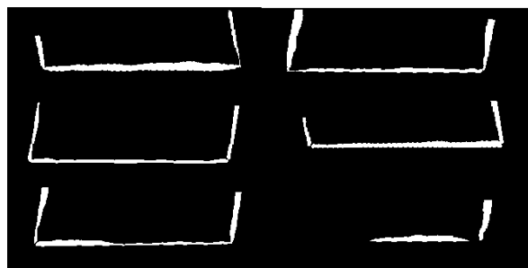
Figure 4: Dataset example.
